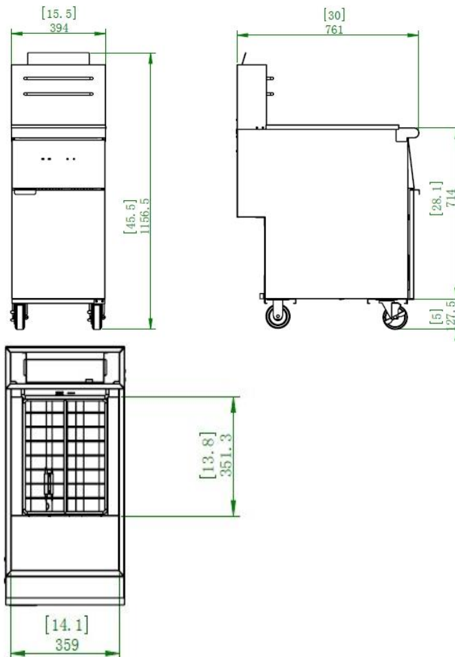
F3 3 Tube Gas Fryer
